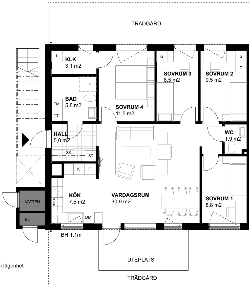
PLAN 1, MARKPLAN
