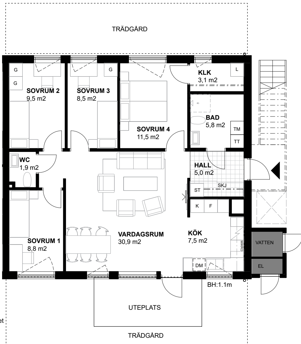
PLAN 1, MARKPLAN
