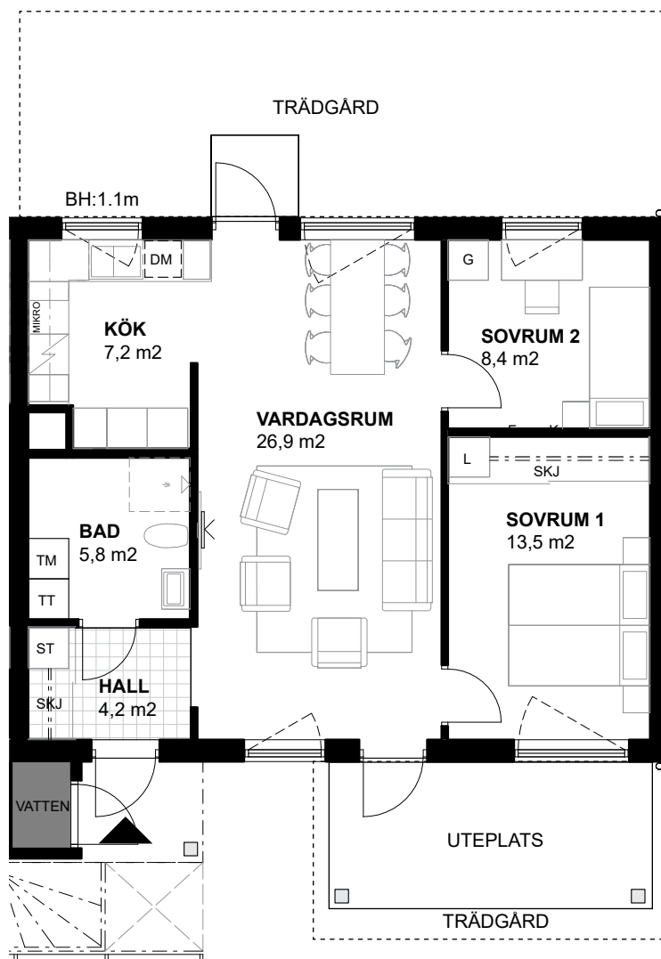
PLAN 1, MARKPLAN
