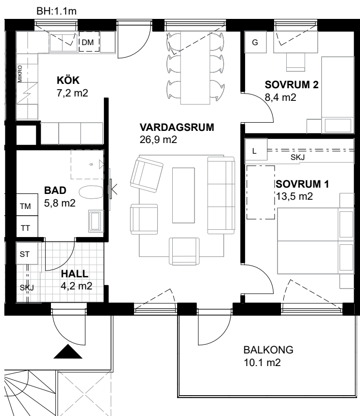
PLAN 2
